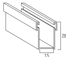
Guida in alluminio A14 GUIAL..14M 15 x 28 mm
