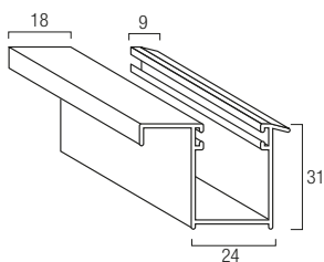
Guida in alluminio A31 GUAL..31M 24 x 31 mm
