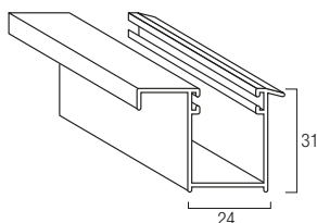
Guida in alluminio A31 GUAL..31M 24 x 31 mm
