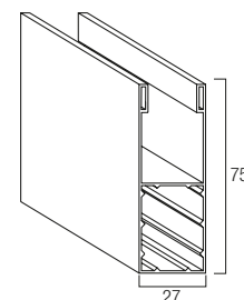
Guida in alluminio A75 GUAL..75M 27 x 75 mm
