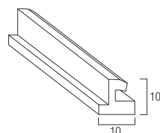
Terminale in gomma TERPVCAL 10 x 10 mm
