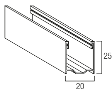
Guida in alluminio A25 GUIAL..25M 20 x 25 mm
