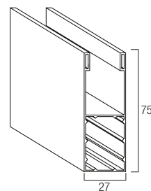
Guida in alluminio A75 GUIAL..75M 27 x 75 mm
