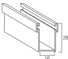
Guida in alluminio A16 GUAL..16M 16 x 28 mm
