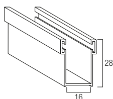
Guida in alluminio A16 GUIAL..16M 16 x 28 mm
