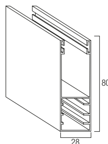
Guida in alluminio A80 GUAL..80M 28 x 80 mm
