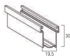
Guida in alluminio A30 GUAL..30M 19,5 x 30 mm
