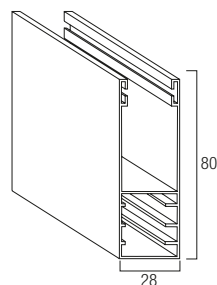
Guida in alluminio A80 GUIAL..80M 28 x 80 mm
