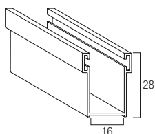
Guida in alluminio A16 GUIAL..16M 16 x 28 mm
