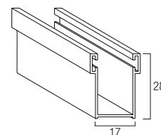
Guida in alluminio A28 GUAL..28M 17 x 28 mm
