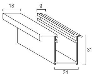
Guida in alluminio A31 GUIAL..31M 24 x 31 mm
